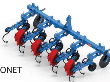
ECONET SGI
